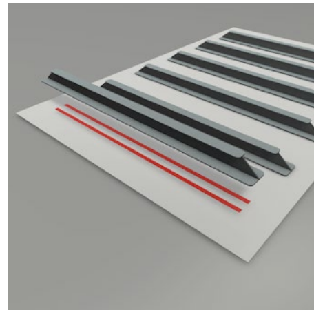
Metal Stiffener Bonding
